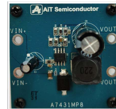
A7431 42V, 125kHz, 3A DC-DC Step-Down
