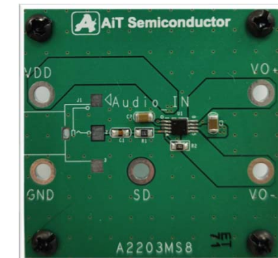
A2203 1.1W @8Ω Class=AB Audio Power Amplifier
