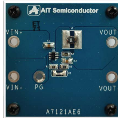
A7121A 1MHz, 2A, 6V DC-DC Buck
